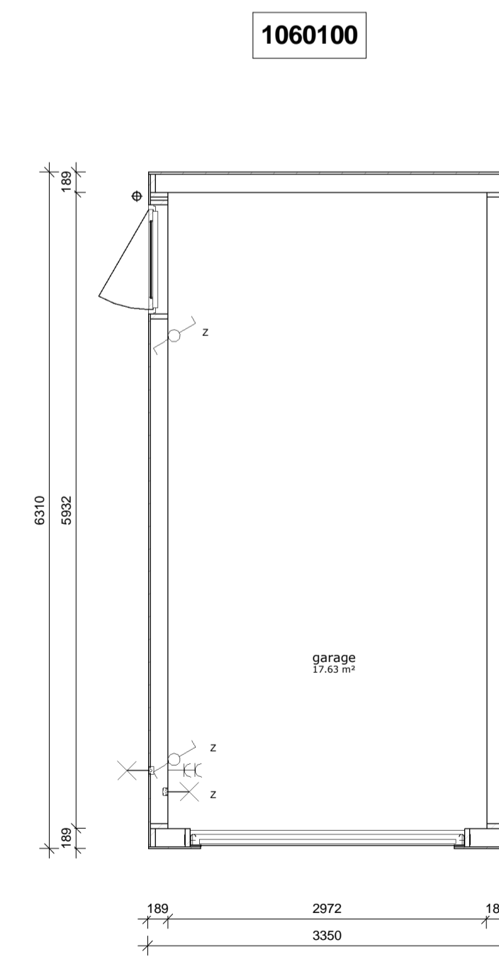
garage
